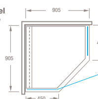
SATURN Tile Channel Drain 905 Neo Angle Left side drain
