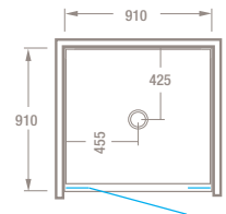
SATURN Tile 910 3 Sided
