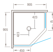
SATURN Tile 905 Neo Angle
