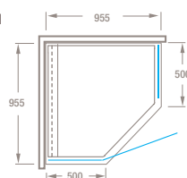
SATURN Tile Channel Drain 955 Neo Angle Left side drain
