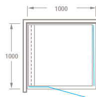
SATURN Tile Channel Drain 1000 2 Sided Left side drain
