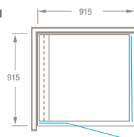
SATURN Tile Channel Drain 915 2 Sided Left side drain
