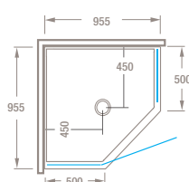
SATURN Tile 955 Neo Angle
