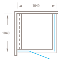
SHAPE Shower Channel Drain 1040 2 Sided
